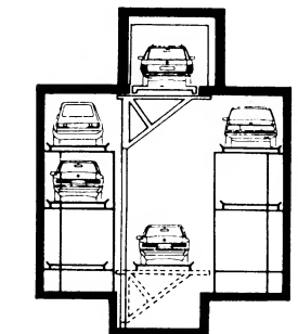
⑭ Parksafes system
